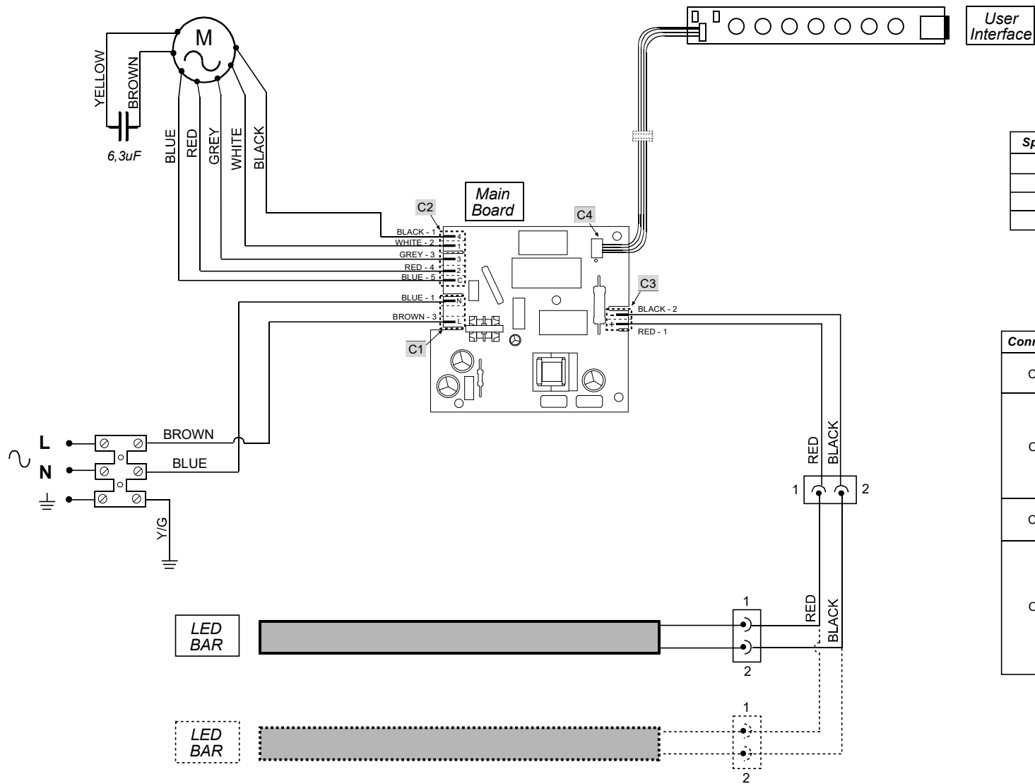
Motor (M) (Family S40 024 xx)
