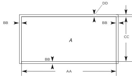
A. Bottom of cabinet cutout without spacers
