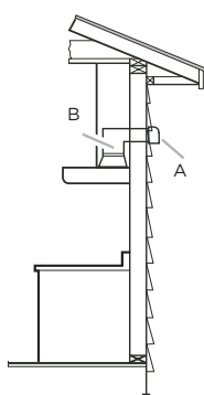
Wall Venting
