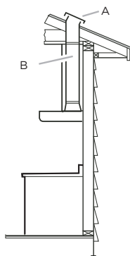
Roof Venting
